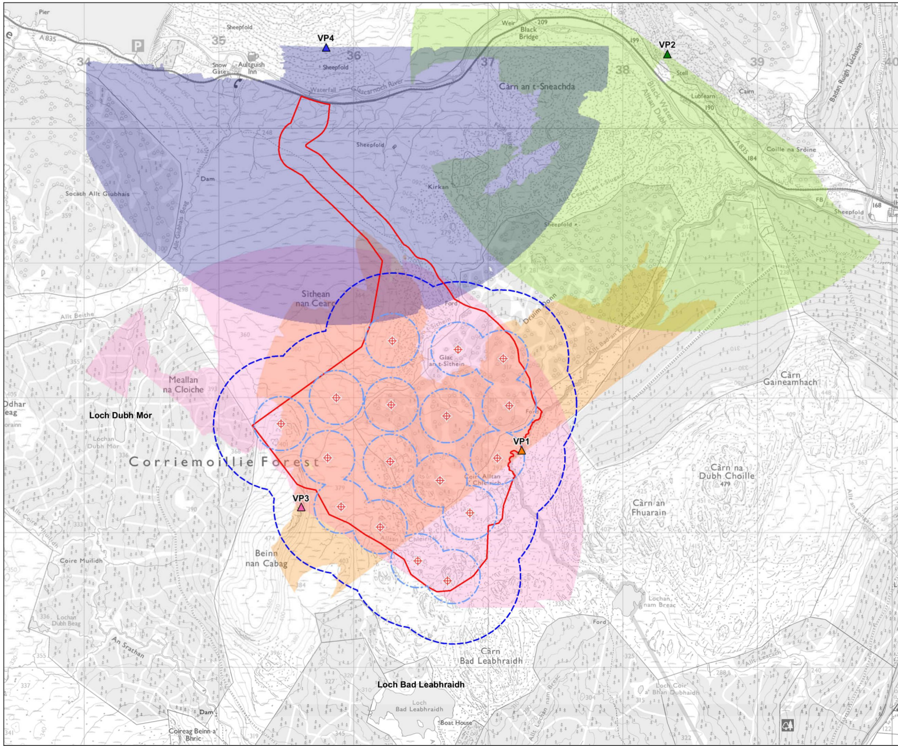
Figure 7.2 - VP Flight Activity Survey Plan Map 1 of 1
